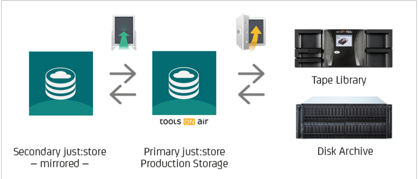
Full just:store and Archiware P5 production setup: P5 Synchronize for data Cloning, P5 Archive for long-term Archiving
